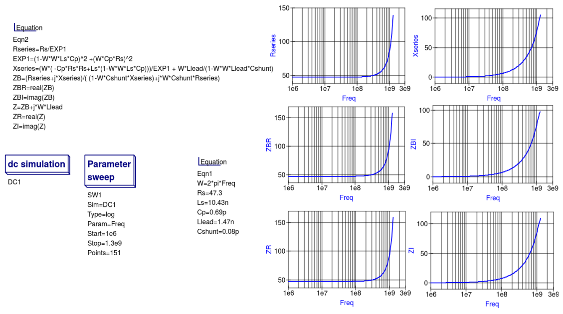
Figure 10: Qucs simulation of nominal 47 Ω resistor based on theoretical analysis.
