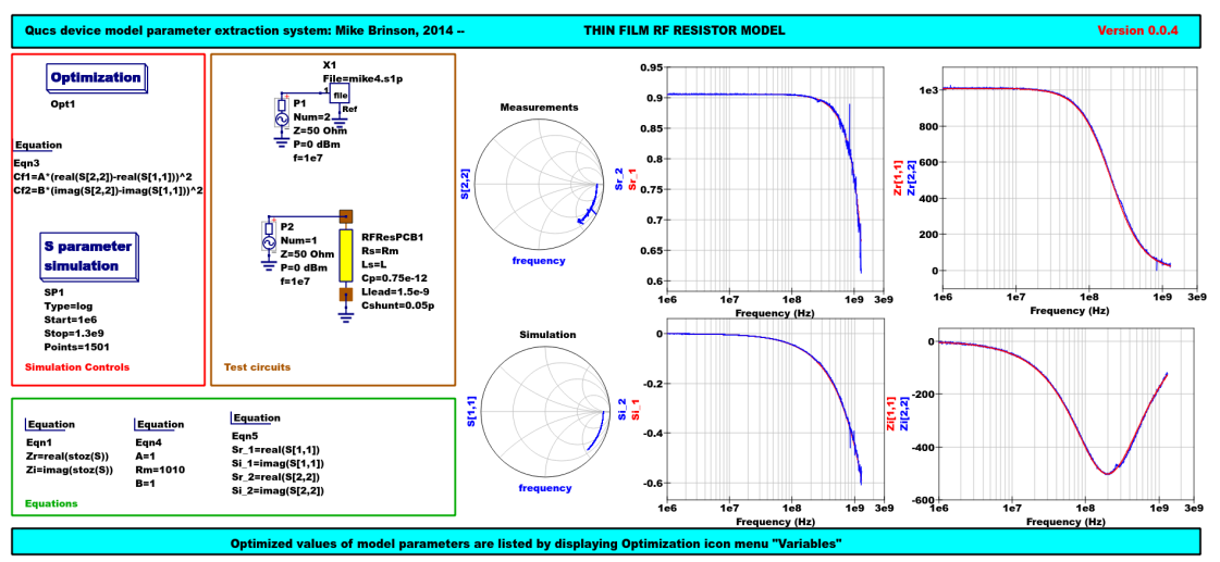
Figure 11: Qucs device model parameter extraction system applied to a nominal 1000 Ω resistor represented by the subcircuit model illustrated in Figure 2 (c).
